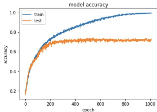
Fig. 6: Accuracy vs Iterations
